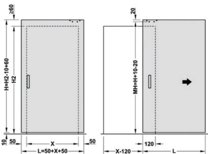
Door installation
