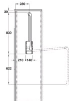
Installed in middle of cabinet side wall
